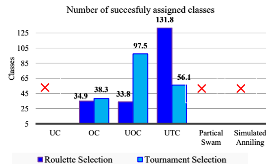
Figure-6: Results of un-preferred classes assigned for a large sized class (200) with soft constraints.
